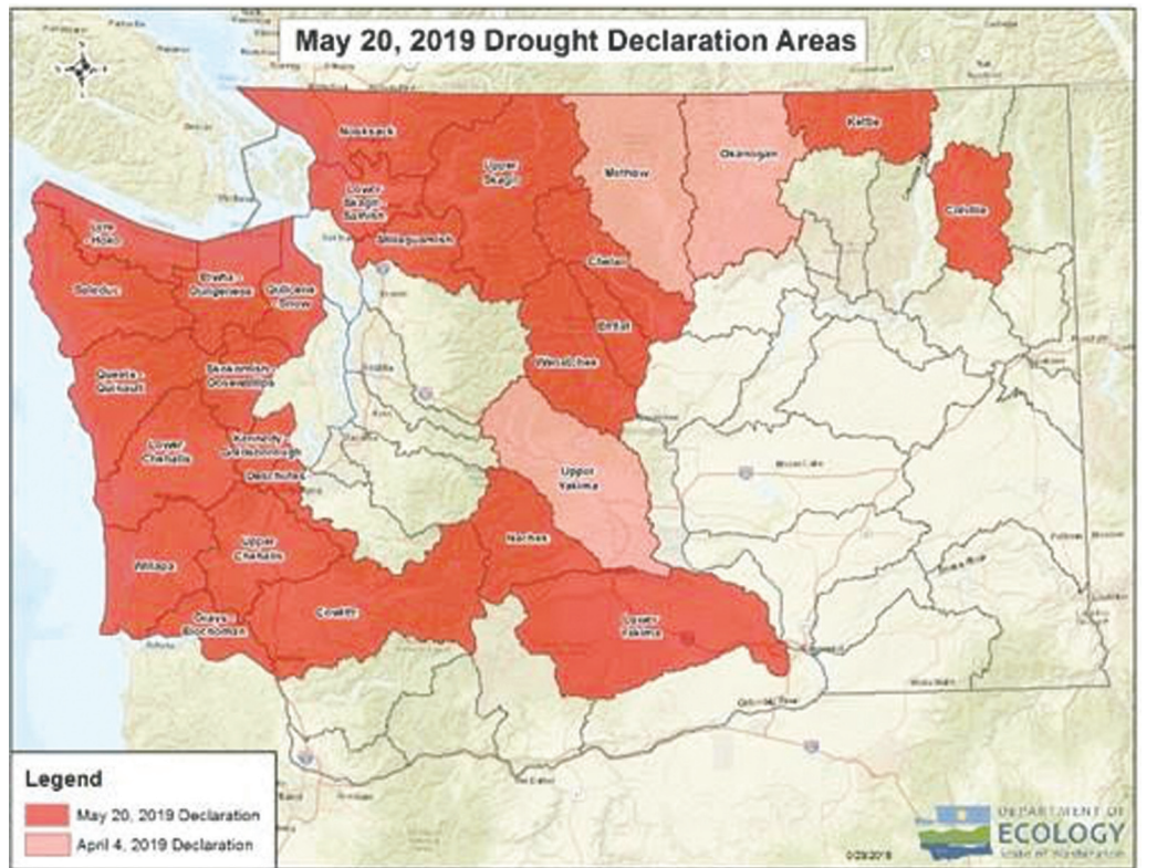
Drought declaration areas of May 20 are shown in red. The three watersheds declared drought areas on April 4, are denoted by the salmon-shaded outlines.
